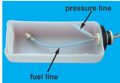
15C - Illustration of fuel line positioning inside cutaway of the tank
