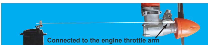
25A- Throttle control rod connected to the engine throttle arm and to the servo arm
