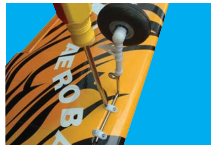
13A- Main landing gear components
