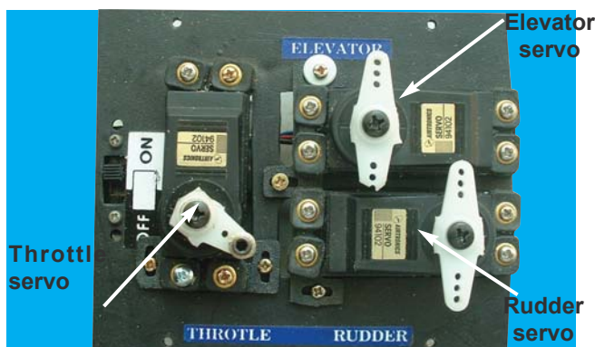
21B- Note the orientation and positions of the three servos in the servo tray
