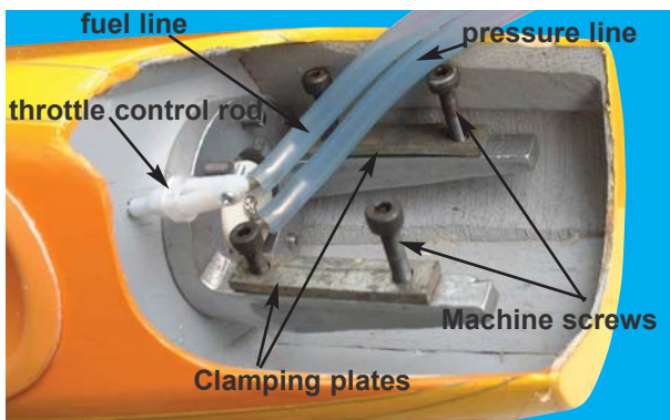
16B- Use a 4mm socket ball wrench or Allen Key to remove the 4 black machine screws that work with the clamping plates on the metal engine mount that has been pre-installed into your Hornet
