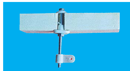
20B- Typical control horn mounted to the surface control
