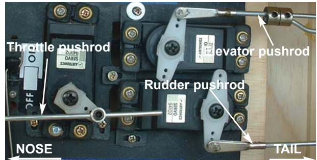
22C- Center the servos, control surfaces & throttle (carb) then connect the control rods to the servos.
