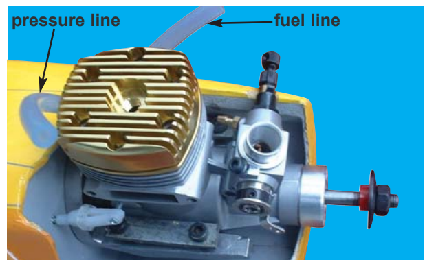
16C- Remove the muffler, position the engine on the engine mount and confirm that the fuel tank metal tubes clear the back of the engine. Trial fit the engine temporarily into place. Tighten the screws only enough to tack the engine into place
