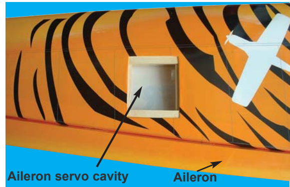
4B- Aileron servo location
