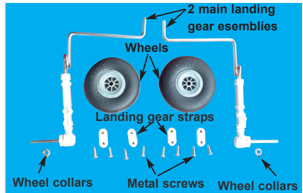
13A- Main landing gear components
