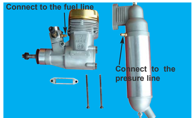
16A- VMAX 46PRO 2 cycle engine recommended
