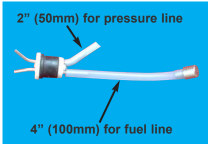
15B - Use 4" (100 mm) for fuel line and 2" (50mm) for pressure line
