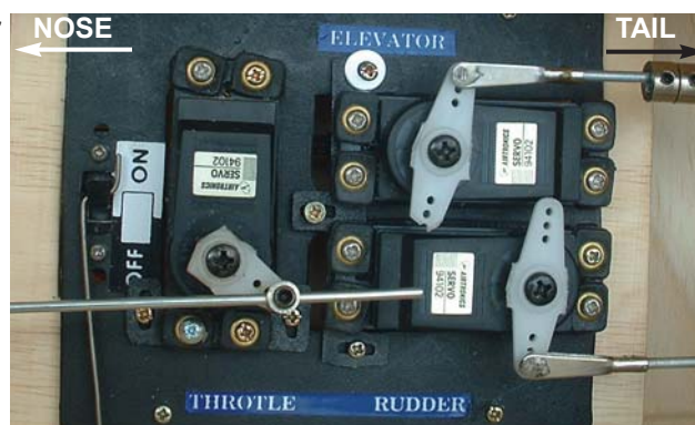
21C- Throttle, rudder and elevator servos connected to their push rods as referenced left to right.
