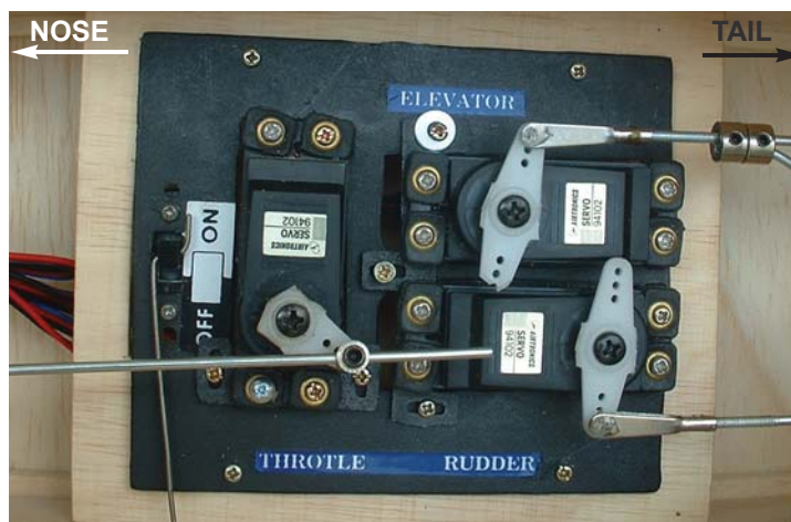
22A- Throttle (left), elevator (upper) & rudder (lower) servos connected to their respective push rods.
