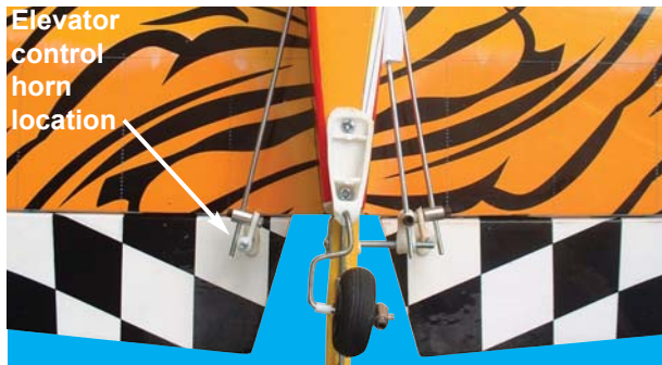
20C- Elevator control horn location
