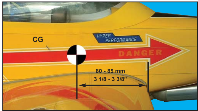
33A- CG location
