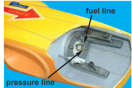
15D - Fuel tank installed into the fuselage
