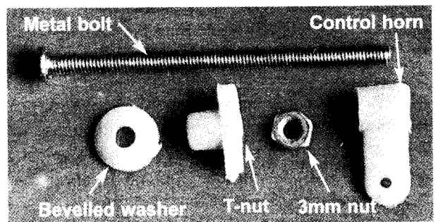
Rudder and tail wheel control system
