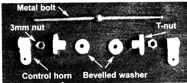
Rudder control horn assembly
