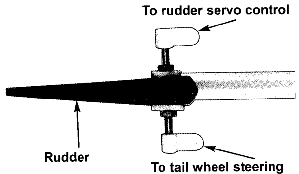
Rudder and tail wheel control system
