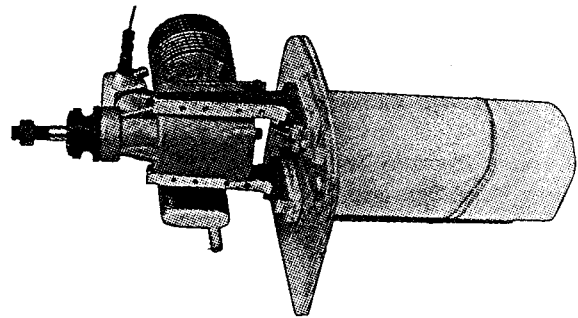
Power module with engine and fuel tank assembly
